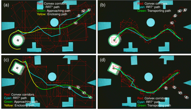
Fig. 17. The path planning results for square and circular objects: (a), (b) The path planning results for the circular object; (c), (d) The path planning results for the square object.
