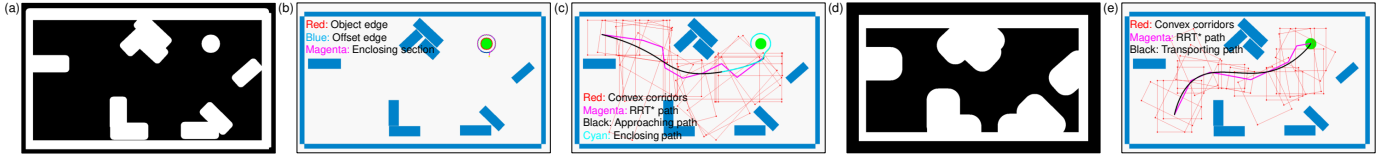
Fig. 10. Path planning for the simulation of transporting a single object: (a) The inflated occupancy map for the approaching and enclosing steps; (b) The generation of object enclosing section; (c) The path planning results for approaching and enclosing the object; (d) The inflated occupancy map for the transporting step; (e) The path planning results for the transporting step.
