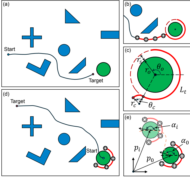
Fig. 6. Path planning for different stages: (a) approaching the object; (b) enclosing the object; (c) obtaining the goal point of the approaching path and the section of enclosing the object; (d) transporting the object; (e) computing the shape of the tube-connected robots at each transport step.
