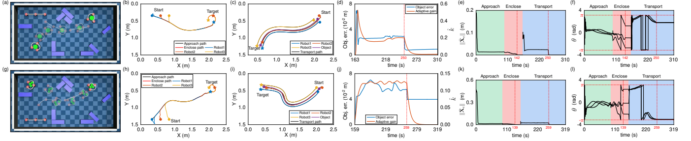
Fig. 11. Simulation results for centralized control: (a), (g) Snapshots of the simulations; (b), (h) Robots' trajectories in the approaching and enclosing steps; (c), (i) Robots' and object's trajectories in the transporting step; (d), (j) Position errors of objects and Adaptive gain \hat{k} ; (e), (k) Position errors of the robots; (f), (l) Orientations of the robots. Obj. err.: object's position error.
