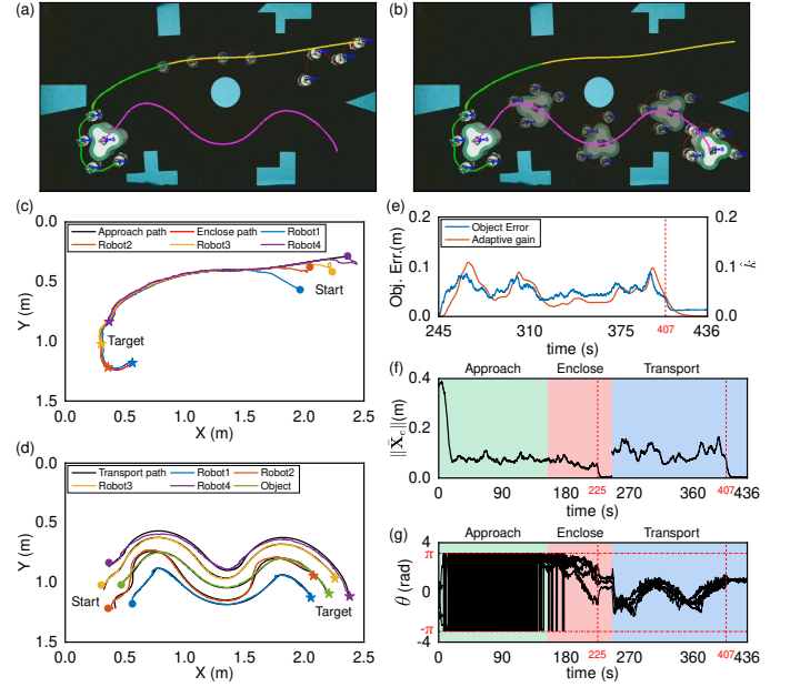
Fig. 16. Experiments of cloud-shaped object: (a), (b) Snapshots of the experiment; (c), (d) Robots' trajectories in the experiment; (e) Position error of the object and the adaptive gain \hat{k} ; (f), (g) Position errors and orientations of the robots during the experiments.
