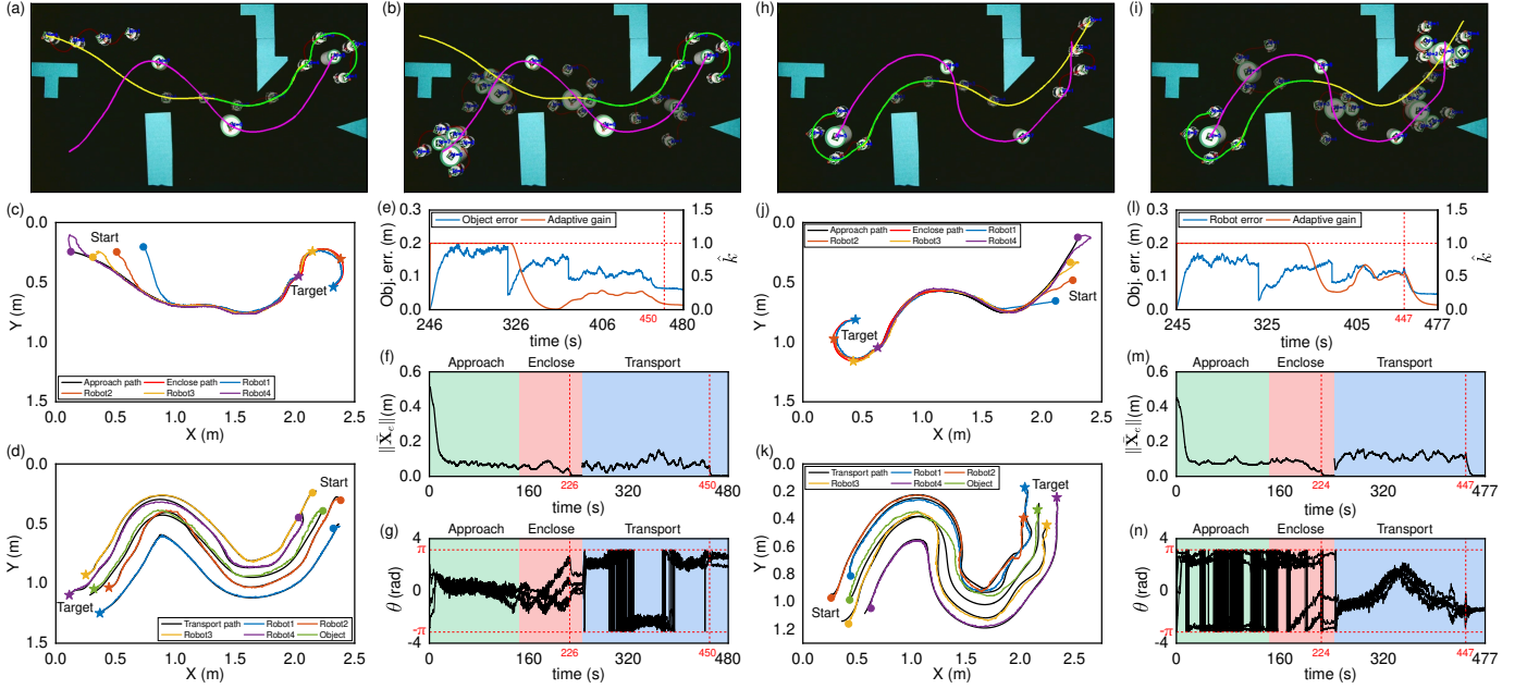
Fig. 22. Experiments of collecting sparse objects: (a), (b) Snapshots of centralized control; (c), (d) Trajectories of the robots with centralized control; (e) Objects' position error with centralized control and the adaptive gain \hat{k} ; (f), (g) Position errors and orientations of the robots with centralized control; (h), (i) Snapshots of distributed control; (j), (k) Trajectories of the robots with distributed control; (l) Objects' position error with distributed control and the adaptive gain \hat{k} ; (m), (n) Position errors and orientations of the robots with distributed control.
