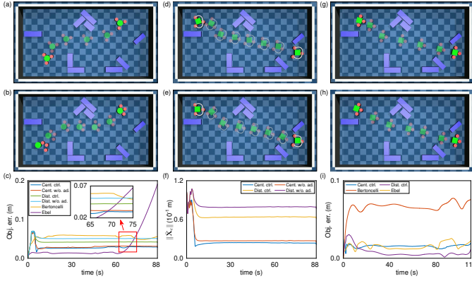
Fig. 13. Comparison and ablation study of the simulation results: (a) (b) Snapshots of Bertoncelli's/Ebel's method with circular object; (c) Position errors of circular objects; (d), (e) Snapshots of the proposed centralized/distributed control with square object; (f) Position errors of robots with different methods; (g), (h) Snapshots of Bertoncelli's/Ebel's method with square object; (i) Position errors of square objects. Cent. ctrl.: centralized control; w/o. ad.: without adaptive gain; Dist.: distributed.
