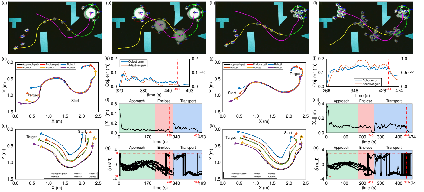
Fig. 20. Experiments of distributed control: (a), (b) Snapshots of the experiment with circular object; (c), (d) Robots' and object's trajectories; (e) Position error of the circular object and the adaptive gain \hat{k} ; (f), (g) Robots' position errors and orientations; (h), (i) Snapshots of the experiment with multiple objects; (j), (k) Robots' and objects' trajectories; (l) Position error of the multiple objects and the adaptive gain \hat{k} ; (m), (n) Robots' position errors and orientations.
