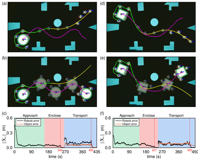
Fig. 18. Experiments of square and circular objects: (a), (b) Snapshots of the experiments with the circular object; (c) Position errors of robots and the circular object; (d), (e) Snapshots of the transporting step for the square-shaped object; (f) Position errors of robots and the square object.
