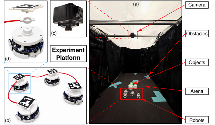
Fig. 14. The platform for the experiments: (a) Overview of the platform; (b) The tube-connected robots; (c) The top-down camera; (d) The customized Mona robot.
