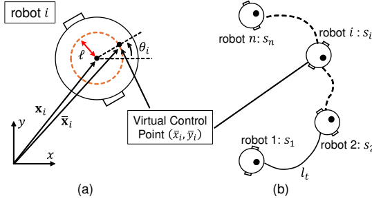
Fig. 2. The configuration of the robot: (a) the original coordinates and the shifted coordinates; (b) the tube-connected robots.
