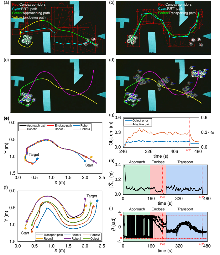
Fig. 19. Experiment of multiple objects: (a), (b) The path planning results for multiple objects; (c), (d) Snapshots of the experiment with multiple objects; (e), (f) Robots' and objects' trajectories during the experiment; (g) The position error of objects and the adaptive gain \hat{k} ; (h), (i) Position errors and orientations of the robots during the experiments.
