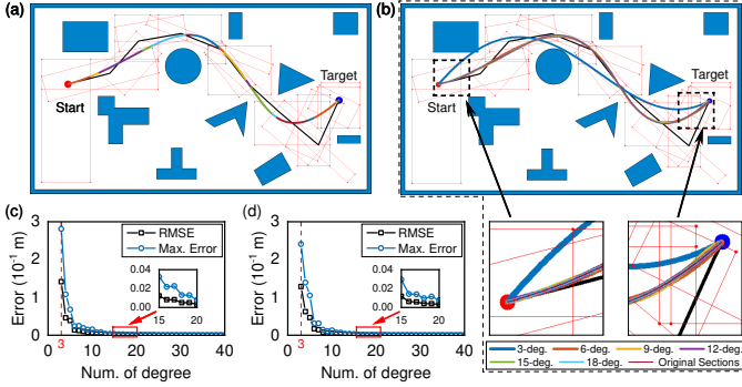
Fig. 7. Validity of the path planning and curve reparametrization: (a) Original piecewise Bézier curve planned by the proposed method; (b) The reparametrized Bézier curve with different degrees; (c) The RMSE and maximum error of the reparametrized curve with different degrees; (d) The RMSE and maximum error of the arc length at different length parameters of the reparametrized curve with different degrees.
