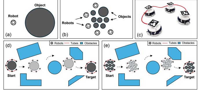
Fig. 1. Conceptual illustration of object transportation by the tube-connected robots: (a) Single robot vs. single object; (b) Multiple robots vs. multiple objects; (c) Tube-connected robots; (d) Tube-connected robots transporting single objects; (e) Tube-connected robots transporting multiple objects.
